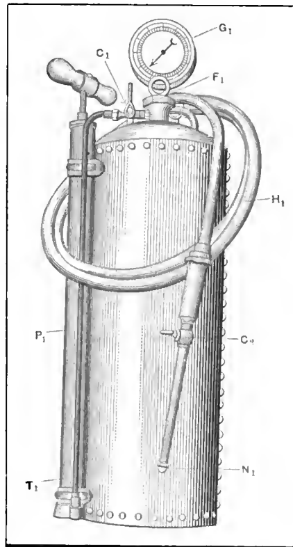
Fig. 3—Rapid engine cleaner
